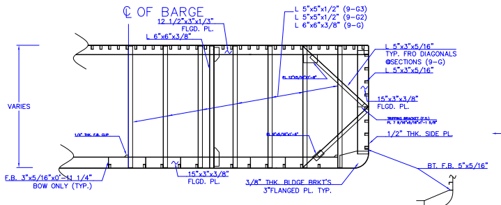
SECTION "9-G" (AS SHOWN) SECTION "9-G2 & G3" (AS NOTED)
