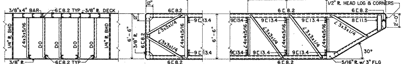
TYP. MID BODY BULKHEAD
