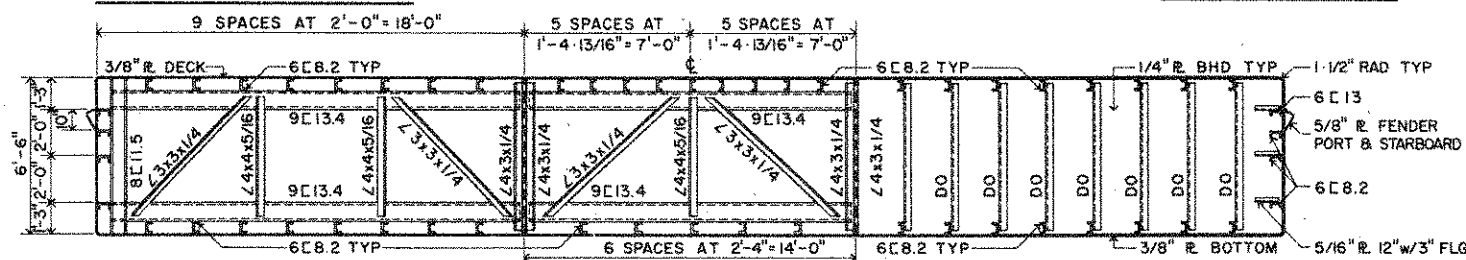
TYP. TRANSVERSE TRUSS
