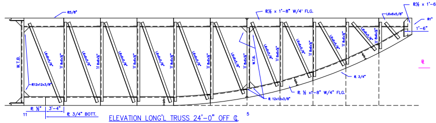
ELEVATION LONG'L TRUSS 24'-0" OFF Q.
