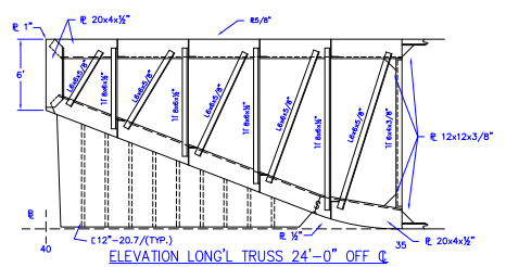
ELEVATION LONG'L TRUSS 24'-0" OFF Q.
