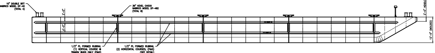
OUTBOARD PROFILE SCALE: 1/8"=1'-0"
