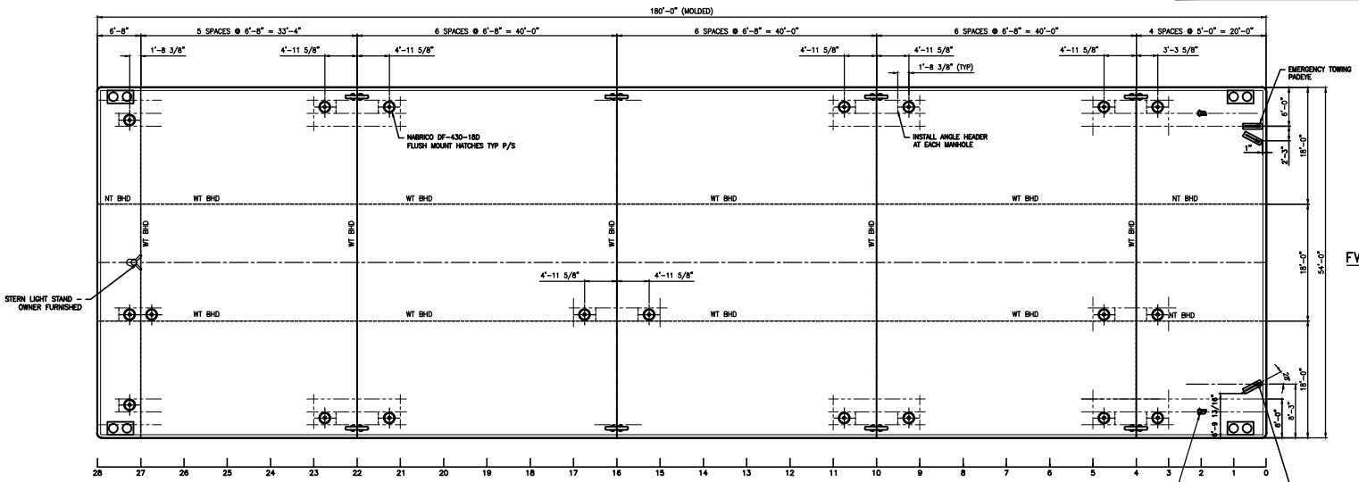
DECK PLAN SCALE: 1/8"=1'-0"
